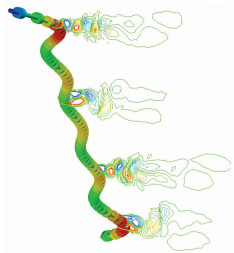
Full-Scale Riser VIV Motion [L/D:10,000]
