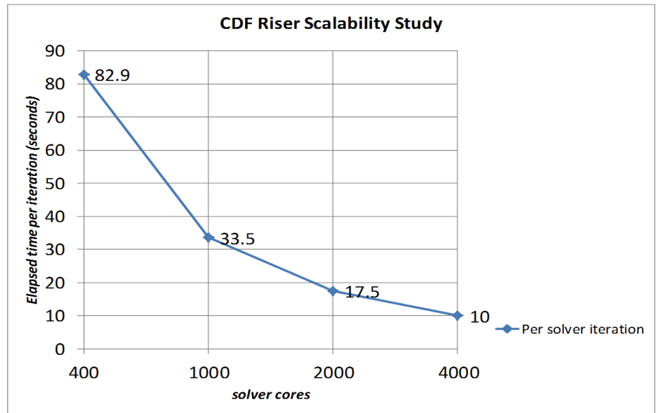
Running AcuSolve for riser simulation on a Cray XC30 system yields dramatic performance improvements, as shown in the chart above.
